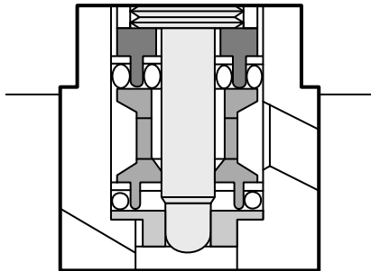
Kel-F® or Teflon® seat eliminates the need for o-ring seal and floating sleeve.
